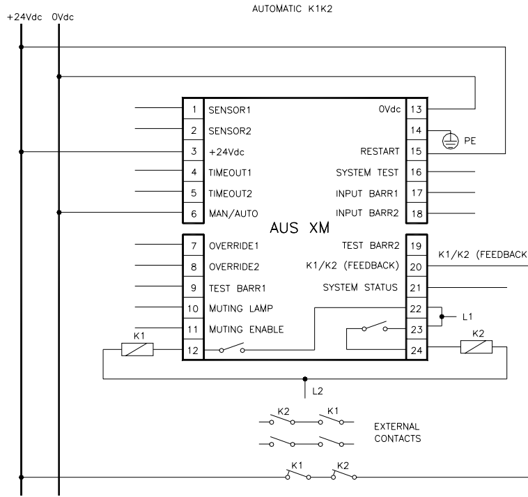
Figure 10 Automatic operation with K1K2 relays
