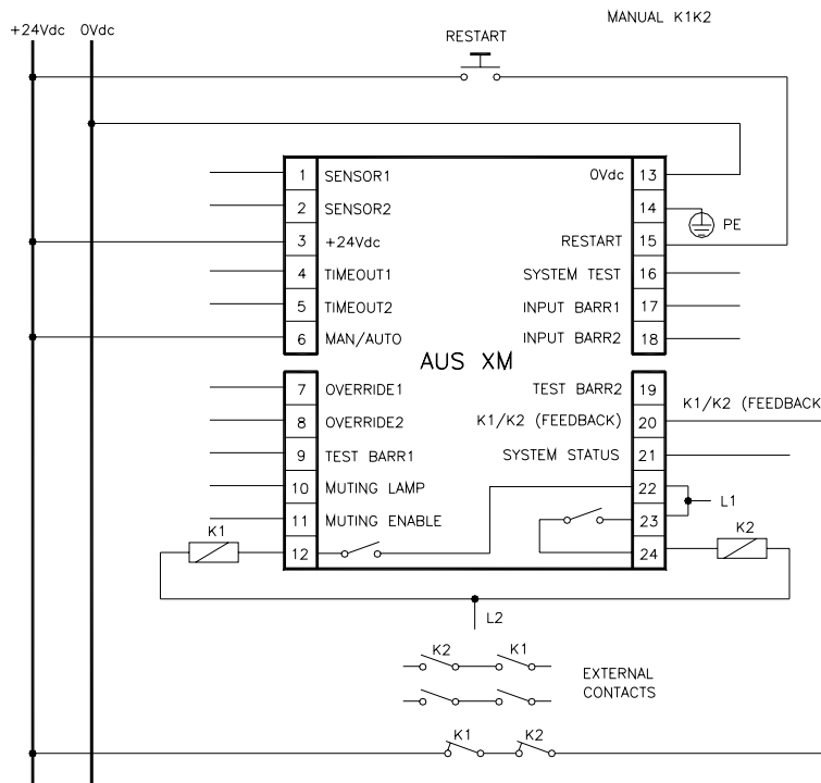
Figure 11 Manual operation with K1K2 relays
