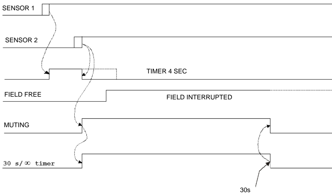
Figure 17 - Muting cycle closed by a timeout
