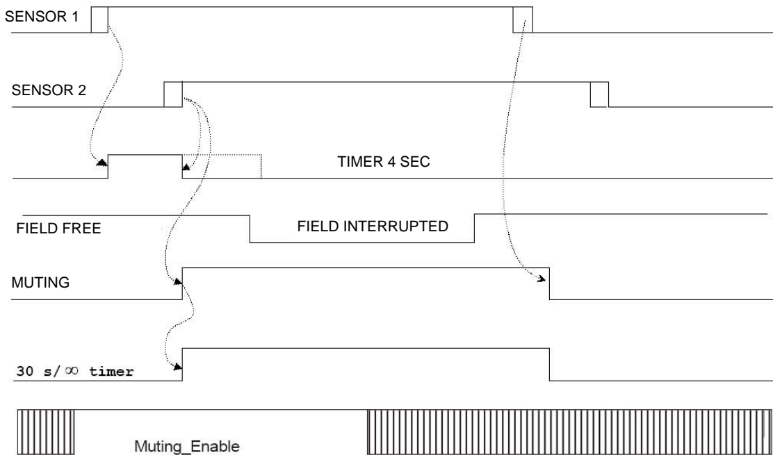
Figure 16 - Muting cycle
