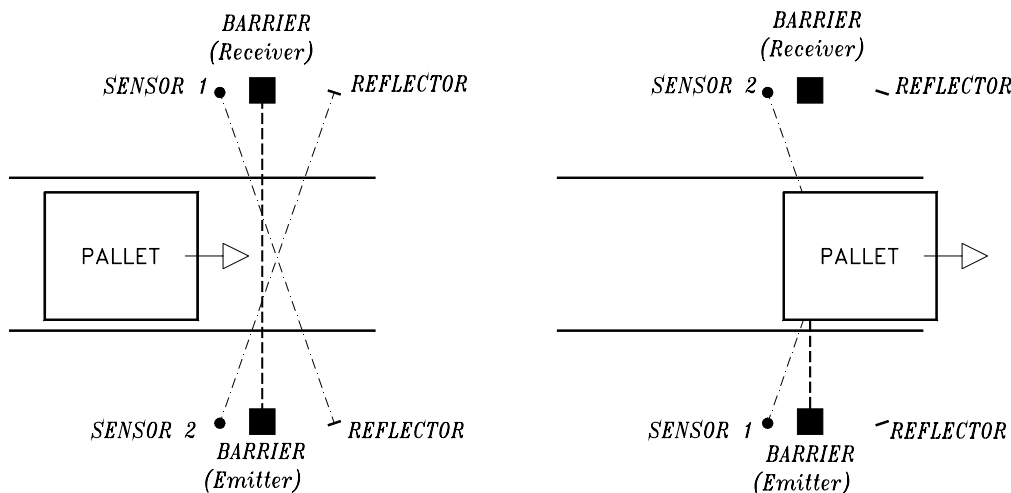
Figure 15 Muting with AUS XM on palletizing system application example
